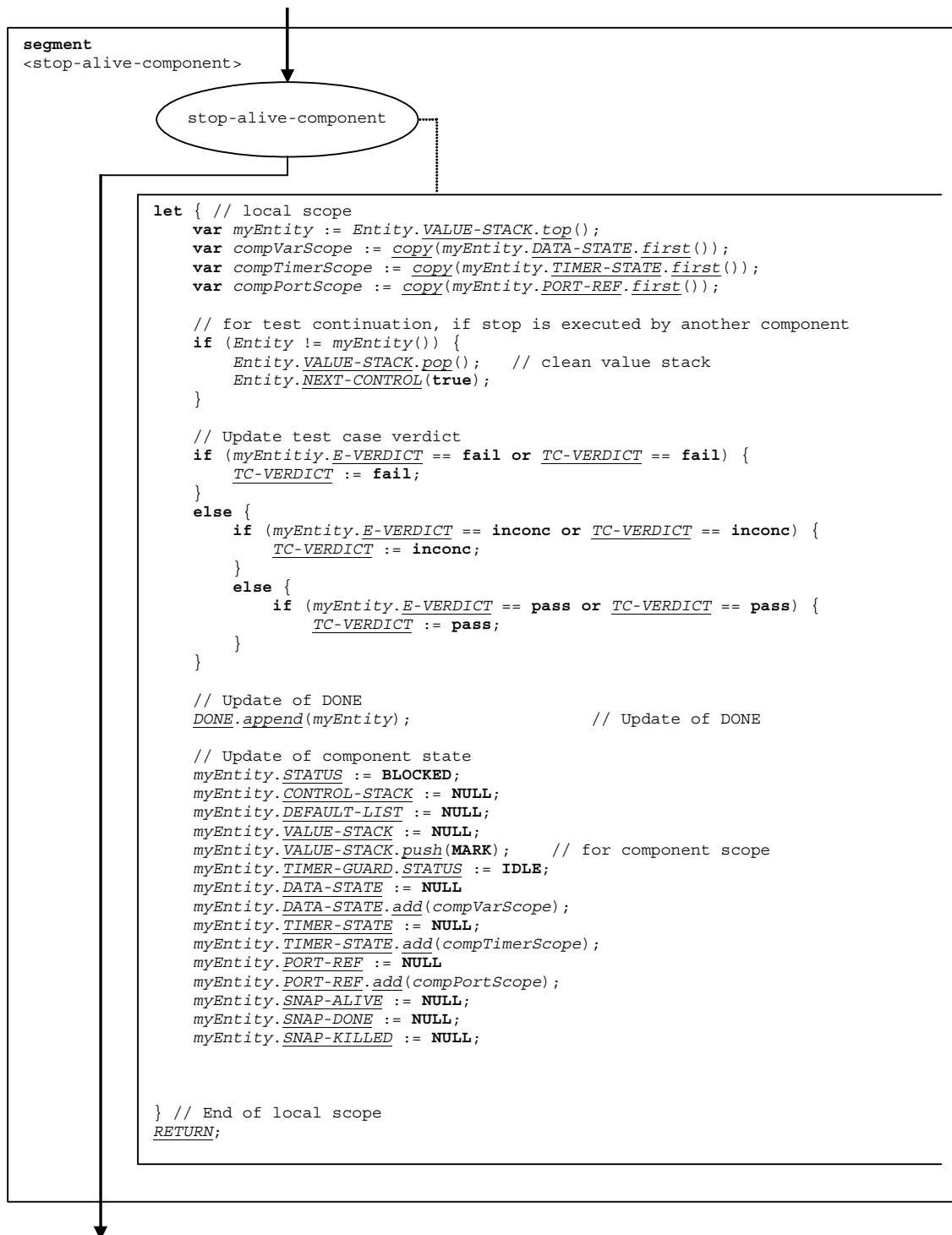
Figure 126: Flow graph segment <stop-component>
