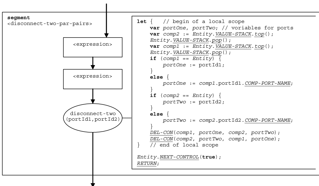
Figure 64e: Flow graph segment &lt;disconnect-two-par-pairs&gt;
